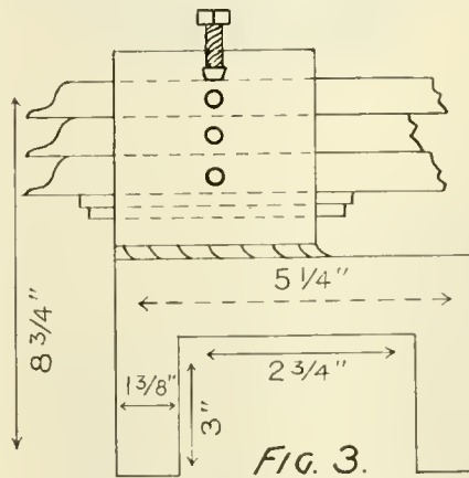
CUTTER FOR CYLINDER AND VALVE PACKING RINGS.
